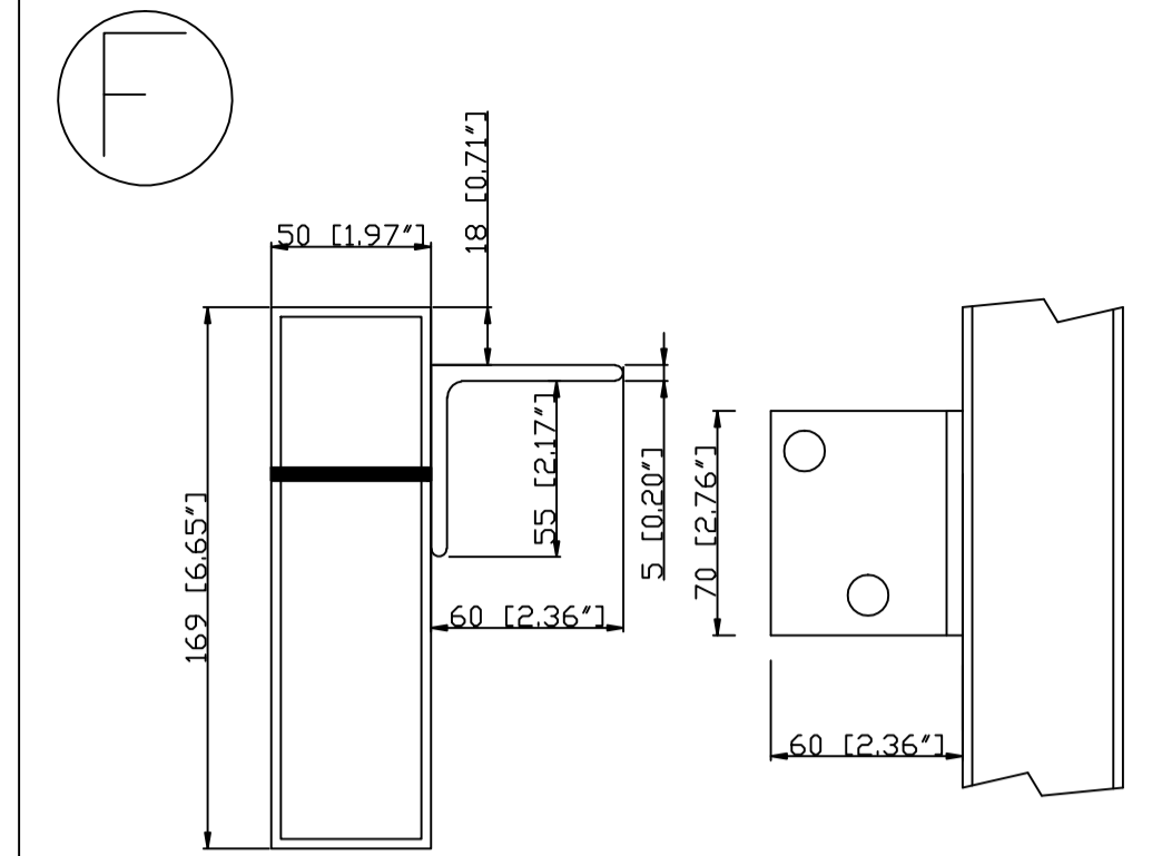
Mounting tabs
